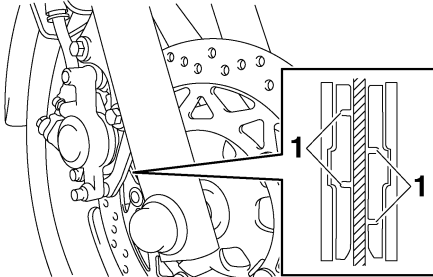
1. Slijtage-indicator remblok
